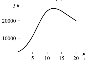
S-I-R model—infected population
