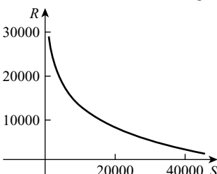
S-I-R model—recovered vs. susceptible
