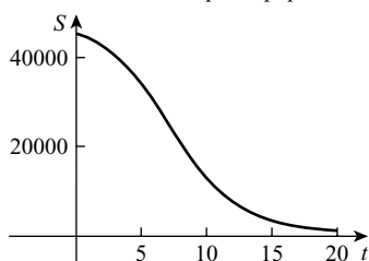
S-I-R model—susceptible population
