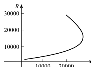
S-I-R model—recovered vs. infected
