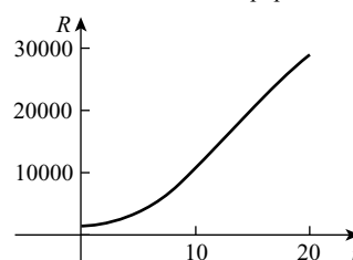
S-I-R model—recovered population
