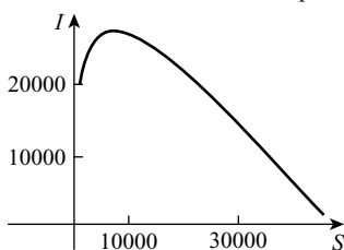
S-I-R model—infected vs. susceptible
